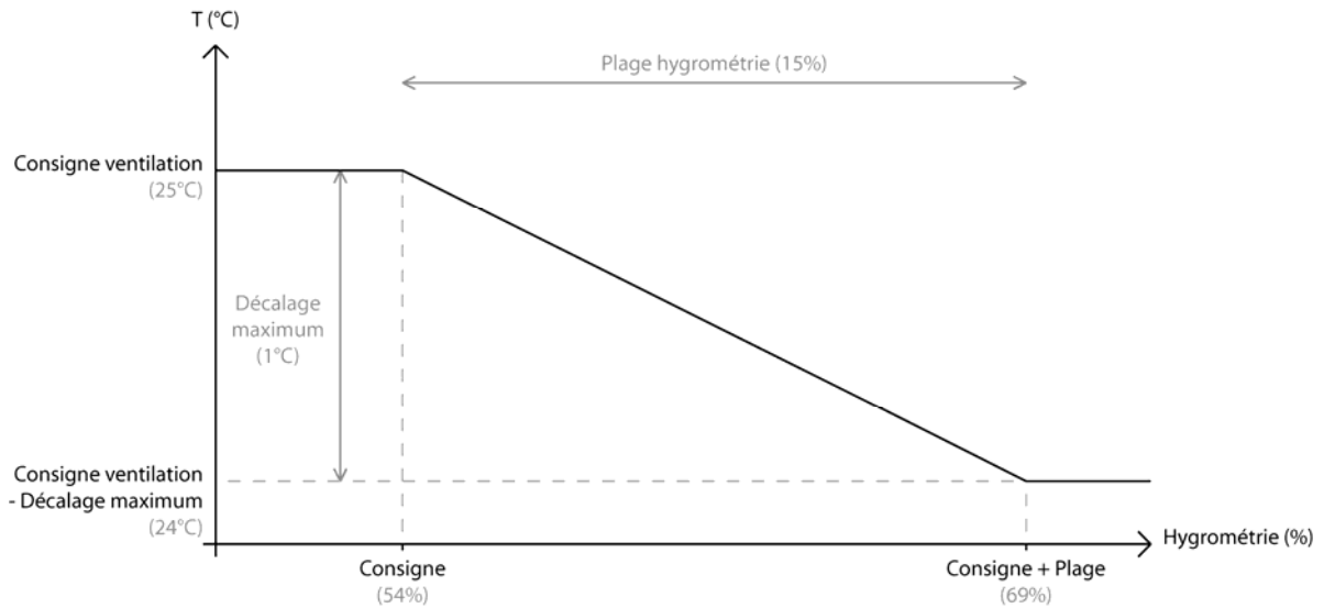
Influence H% 01 / Ventilation
